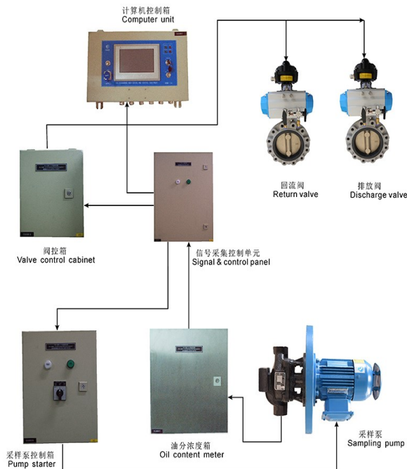
RD-ODME-IIA oil drain monitoring system
